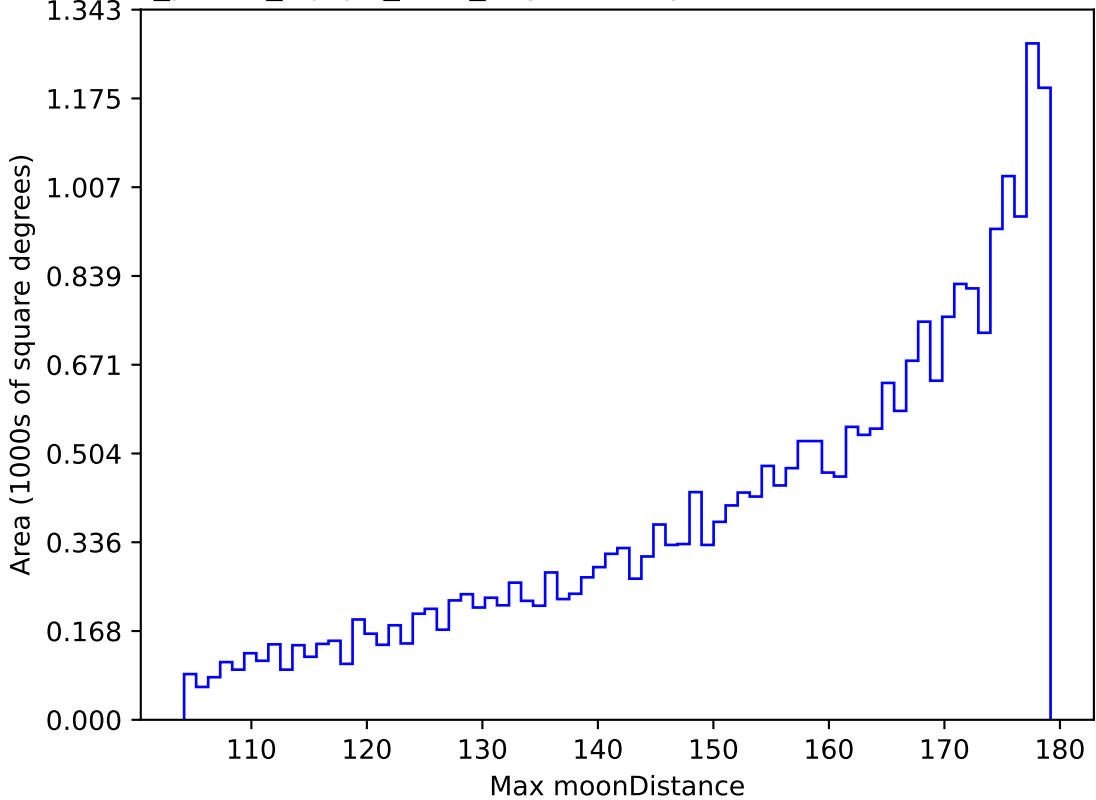
roll_pause_mjdp0_v3.4_10yrs All sky r band: Max moonDistance
