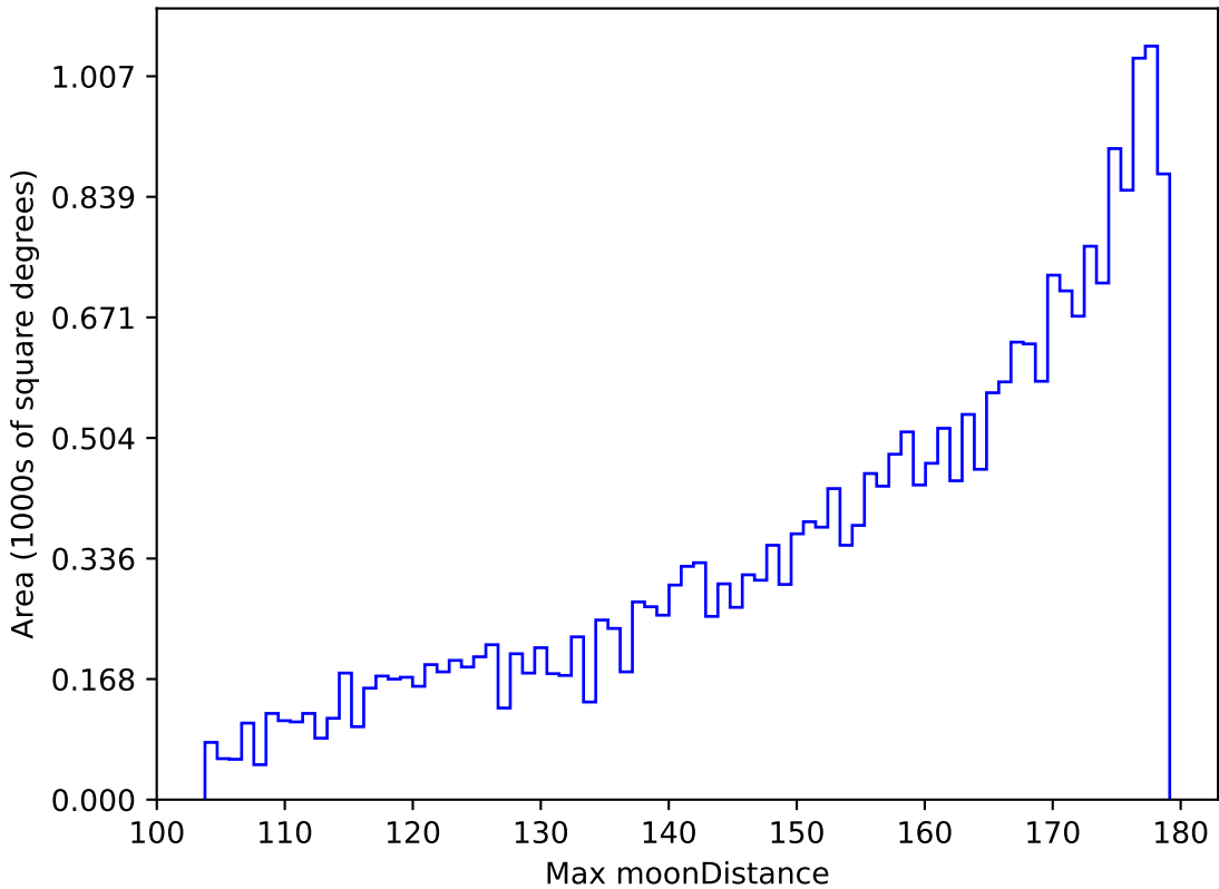
roll_pause_mjdp0_v3.4_10yrs All sky i band: Max moonDistance
