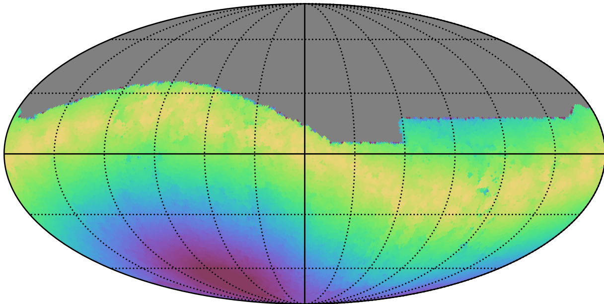
roll_pause_mjdp0_v3.4_10yrs All sky g band: Max moonDistance
