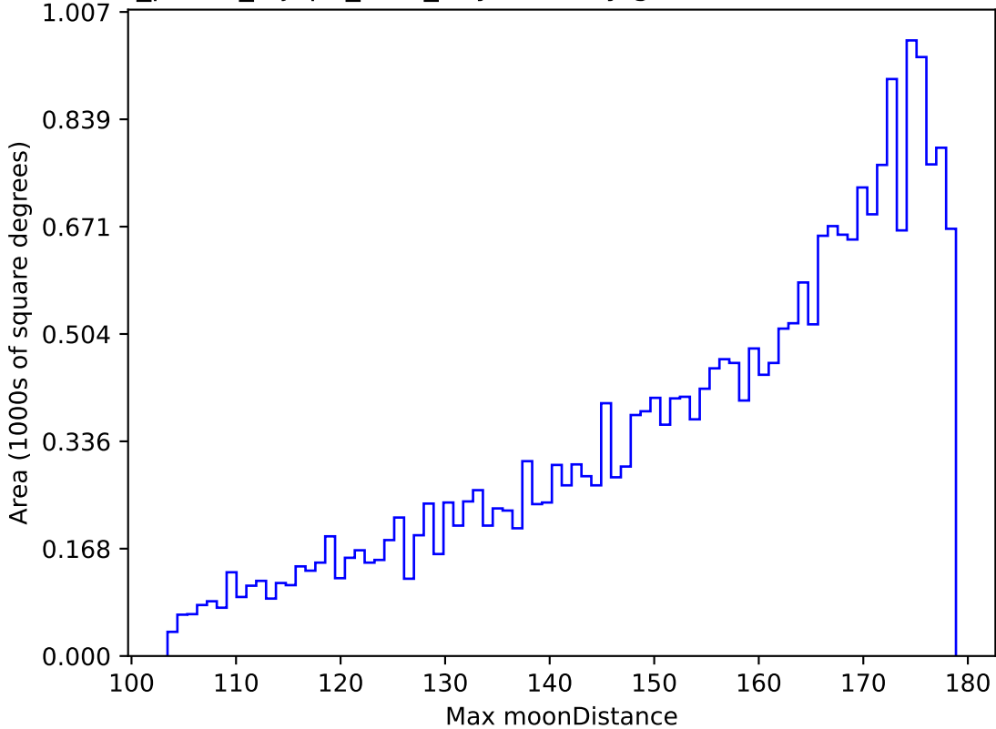
roll_pause_mjdp0_v3.4_10yrs All sky g band: Max moonDistance
