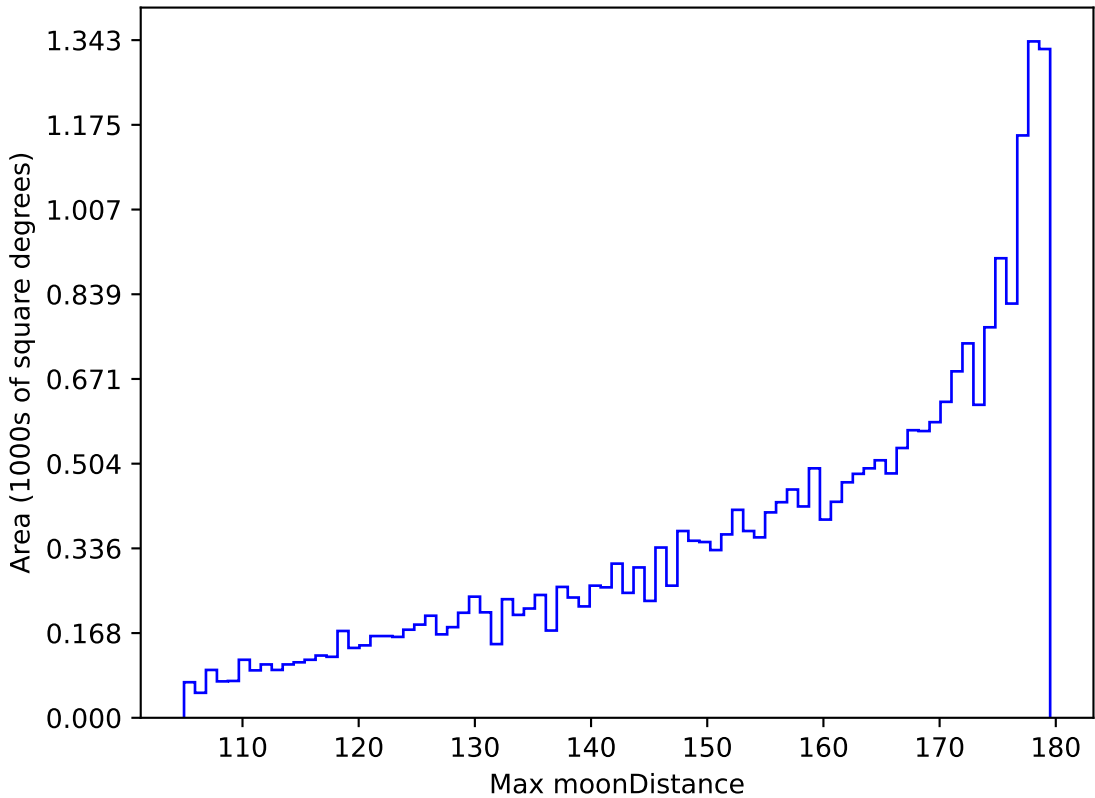
roll_pause_mjdp0_v3.4_10yrs All sky all bands: Max moonDistance
