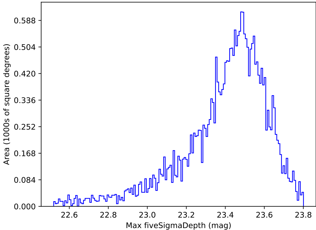
roll_pause_mjdp0_v3.4_10yrs Yr 1 z band: Max fiveSigmaDepth
