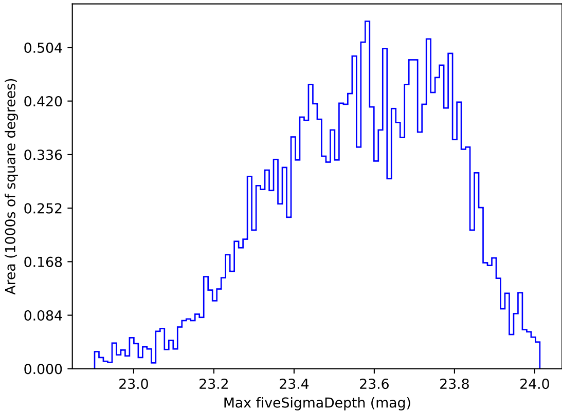
roll_pause_mjdp0_v3.4_10yrs Yr 1 u band: Max fiveSigmaDepth
