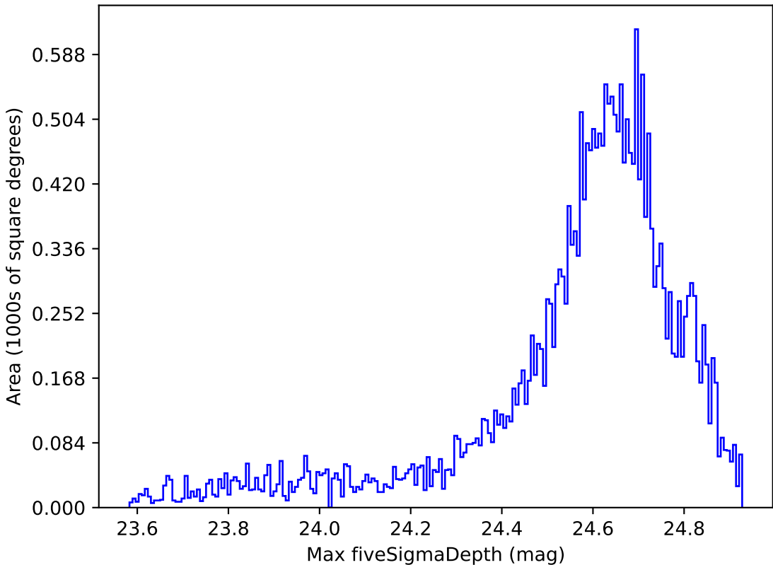
roll_pause_mjdp0_v3.4_10yrs Yr 1 r band: Max fiveSigmaDepth
