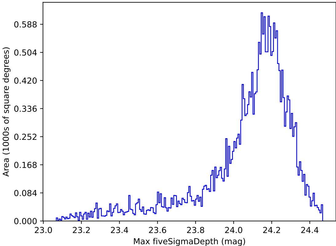
roll_pause_mjdp0_v3.4_10yrs Yr 1 i band: Max fiveSigmaDepth
