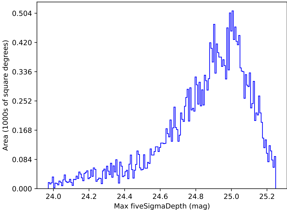
roll_pause_mjdp0_v3.4_10yrs Yr 1 g band: Max fiveSigmaDepth
