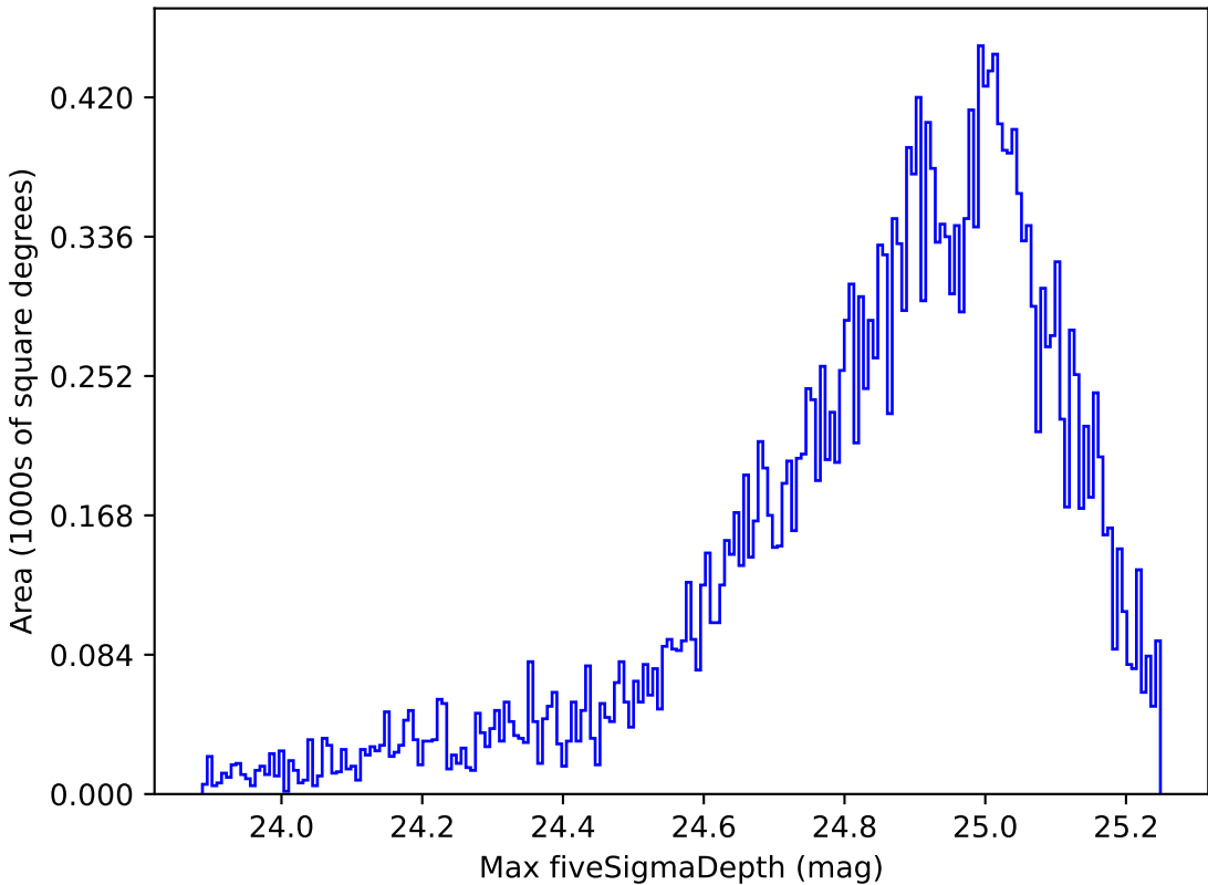
roll_pause_mjdp0_v3.4_10yrs Yr 1 all bands: Max fiveSigmaDepth
