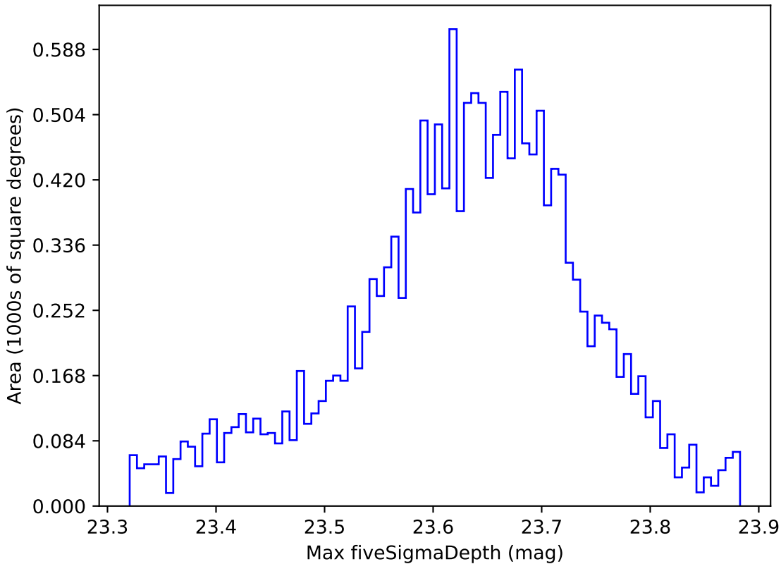
roll_pause_mjdp0_v3.4_10yrs WFD z band: Max fiveSigmaDepth
