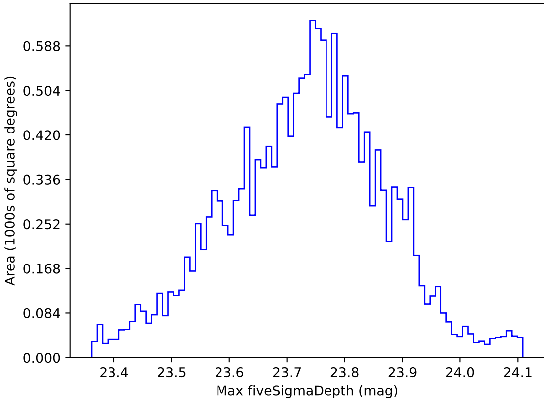
roll_pause_mjdp0_v3.4_10yrs WFD u band: Max fiveSigmaDepth
