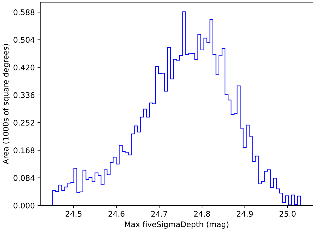
roll_pause_mjdp0_v3.4_10yrs WFD r band: Max fiveSigmaDepth
