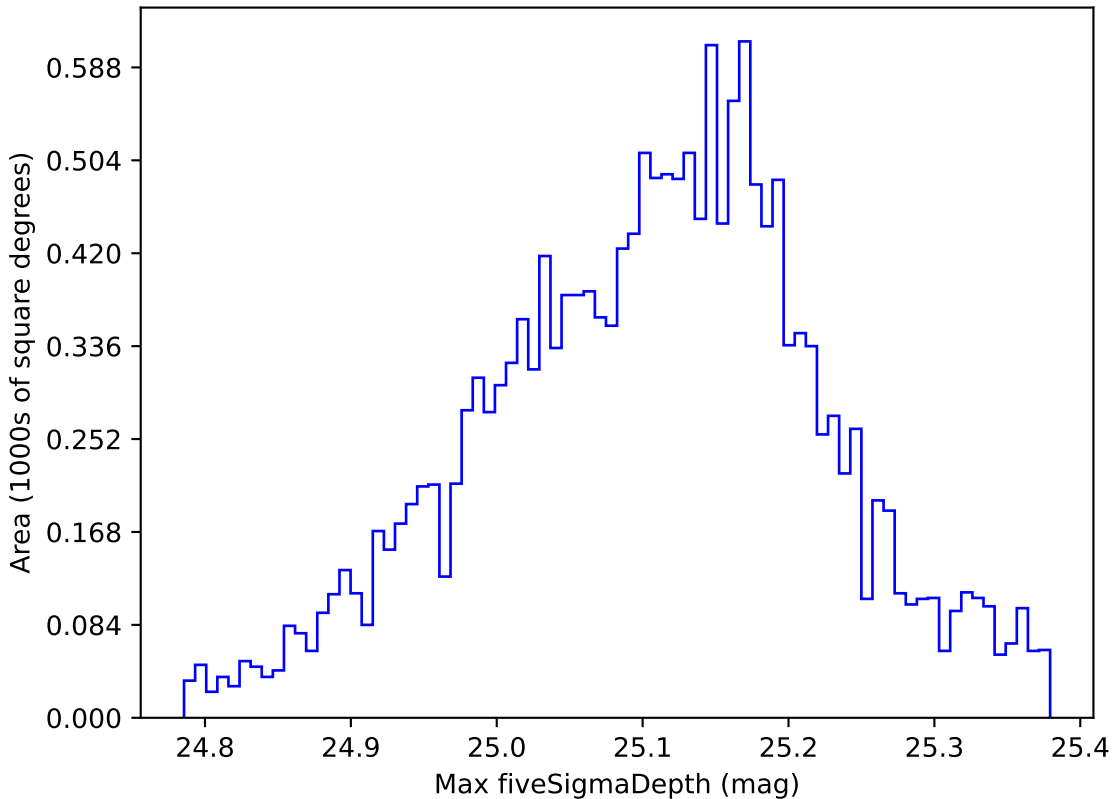
roll_pause_mjdp0_v3.4_10yrs WFD g band: Max fiveSigmaDepth
