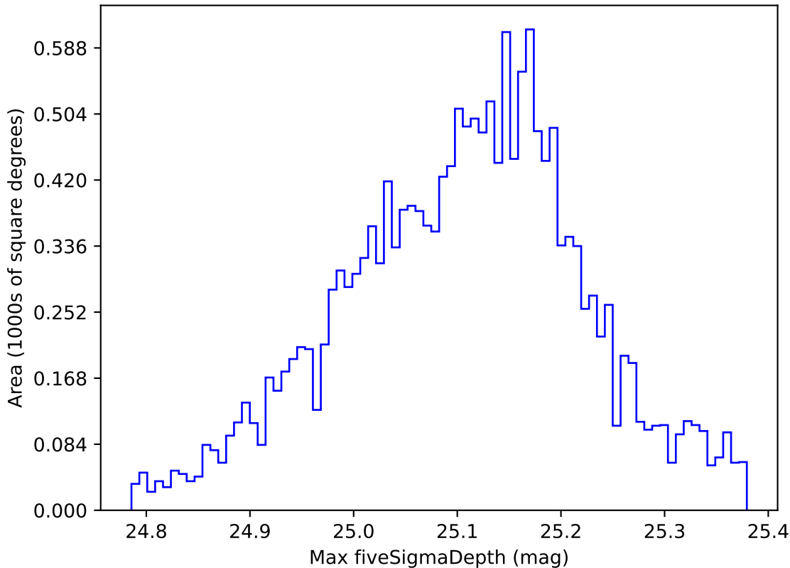
roll_pause_mjdp0_v3.4_10yrs WFD all bands: Max fiveSigmaDepth
