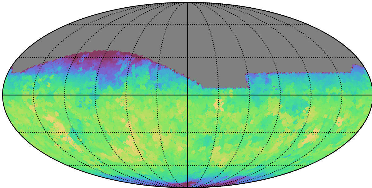
roll_pause_mjdp0_v3.4_10yrs All sky z band: Max fiveSigmaDepth
