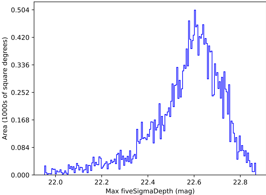
roll_pause_mjdp0_v3.4_10yrs All sky y band: Max fiveSigmaDepth
