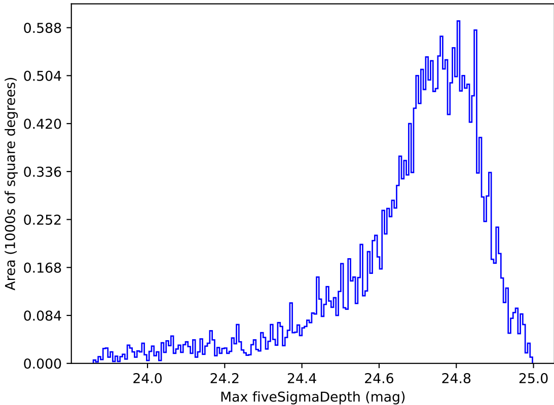
roll_pause_mjdp0_v3.4_10yrs All sky r band: Max fiveSigmaDepth
