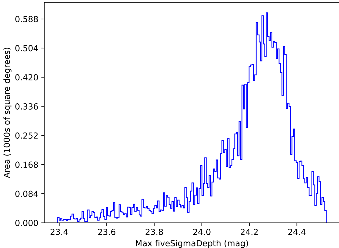
roll_pause_mjdp0_v3.4_10yrs All sky i band: Max fiveSigmaDepth
