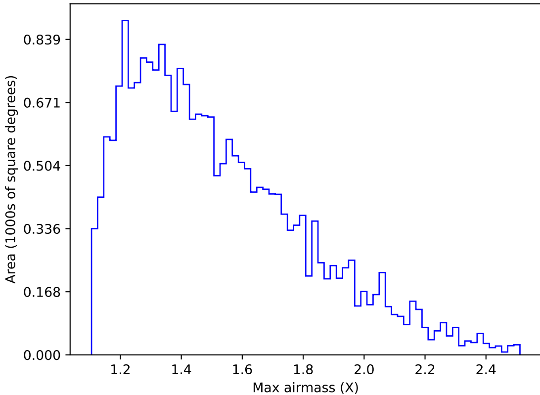
roll_pause_mjdp0_v3.4_10yrs Yr 1 u band: Max airmass
