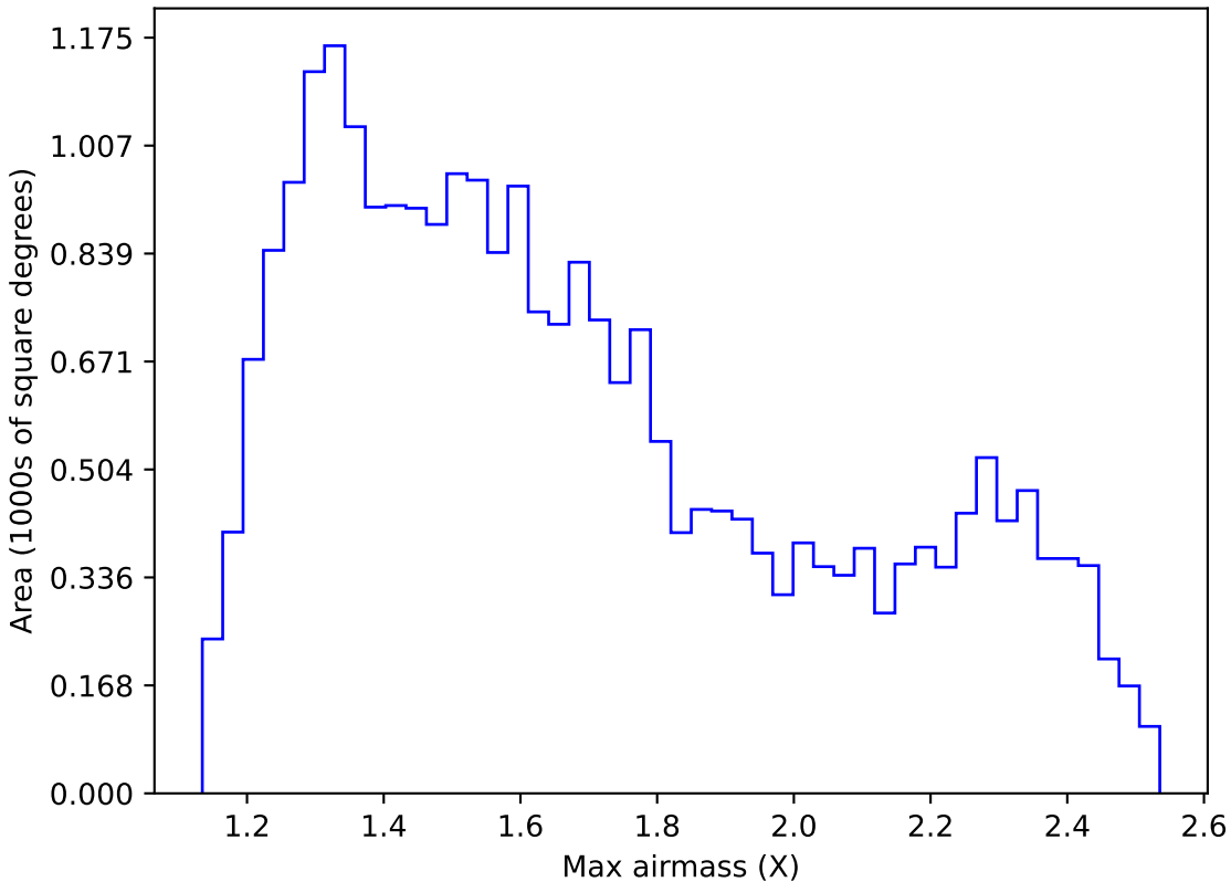
roll_pause_mjdp0_v3.4_10yrs Yr 1 r band: Max airmass
