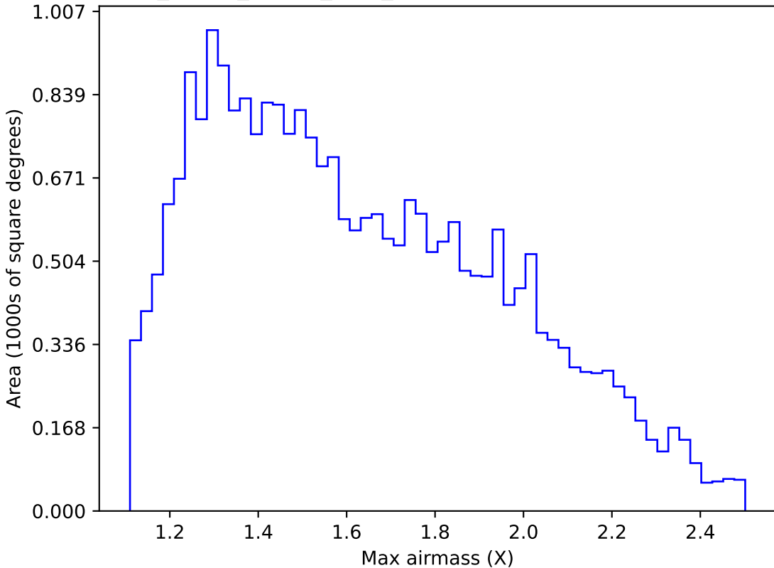
roll_pause_mjdp0_v3.4_10yrs Yr 1 g band: Max airmass
