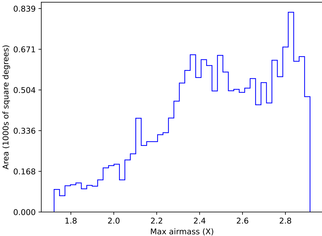
roll_pause_mjdp0_v3.4_10yrs WFD z band: Max airmass
