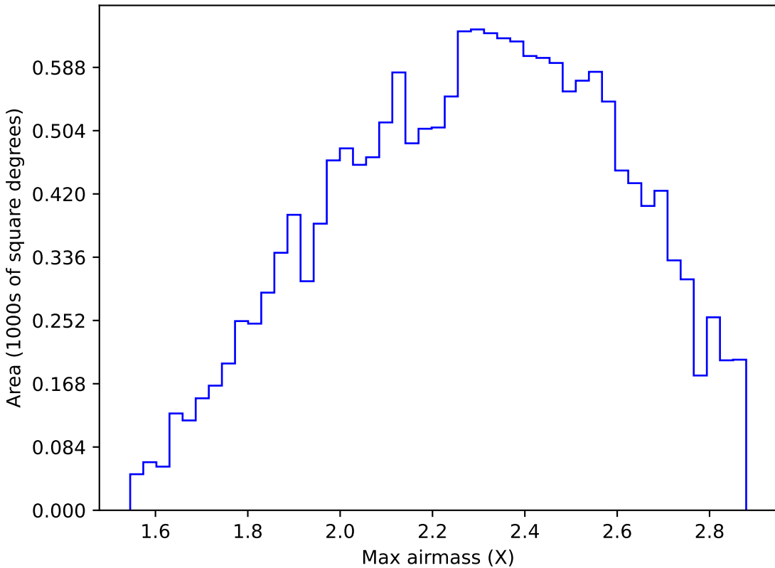
roll_pause_mjdp0_v3.4_10yrs WFD y band: Max airmass
