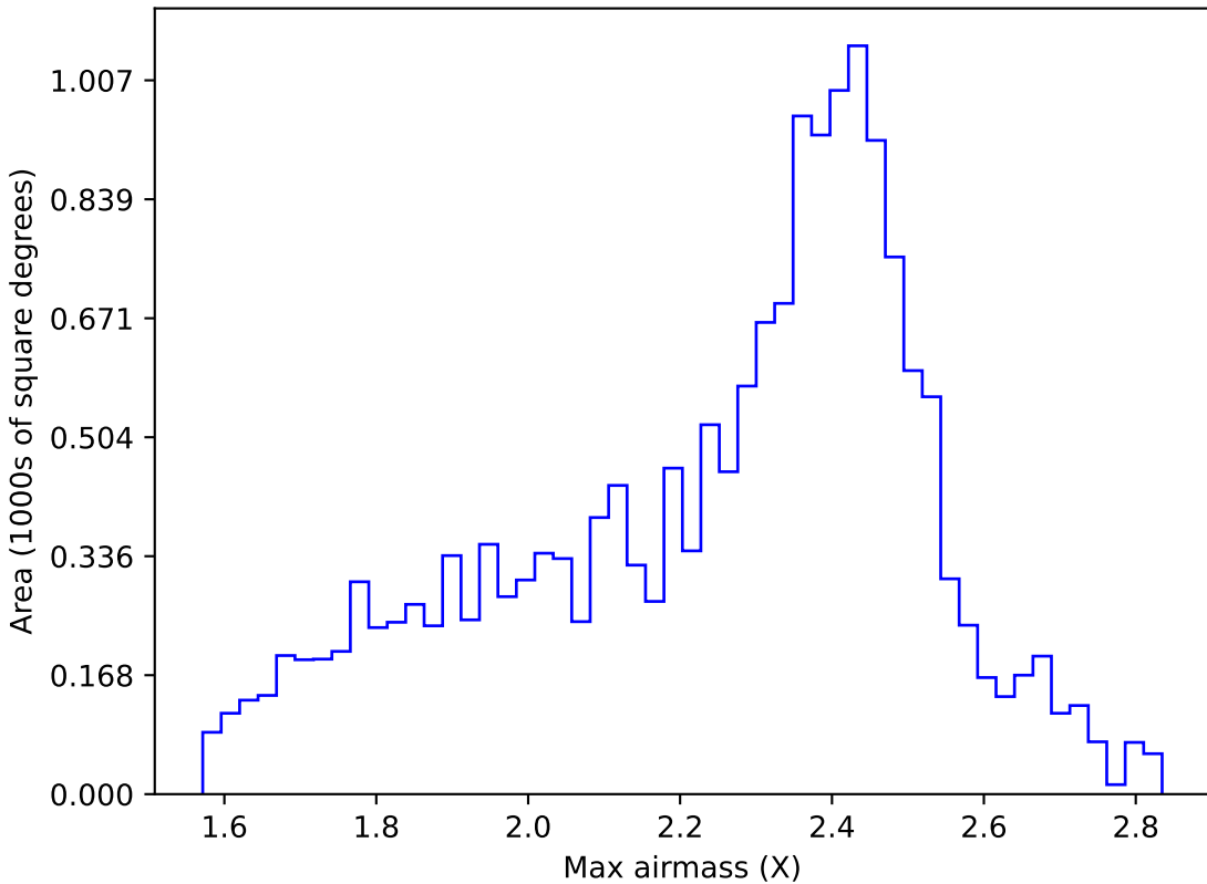
roll_pause_mjdp0_v3.4_10yrs WFD r band: Max airmass
