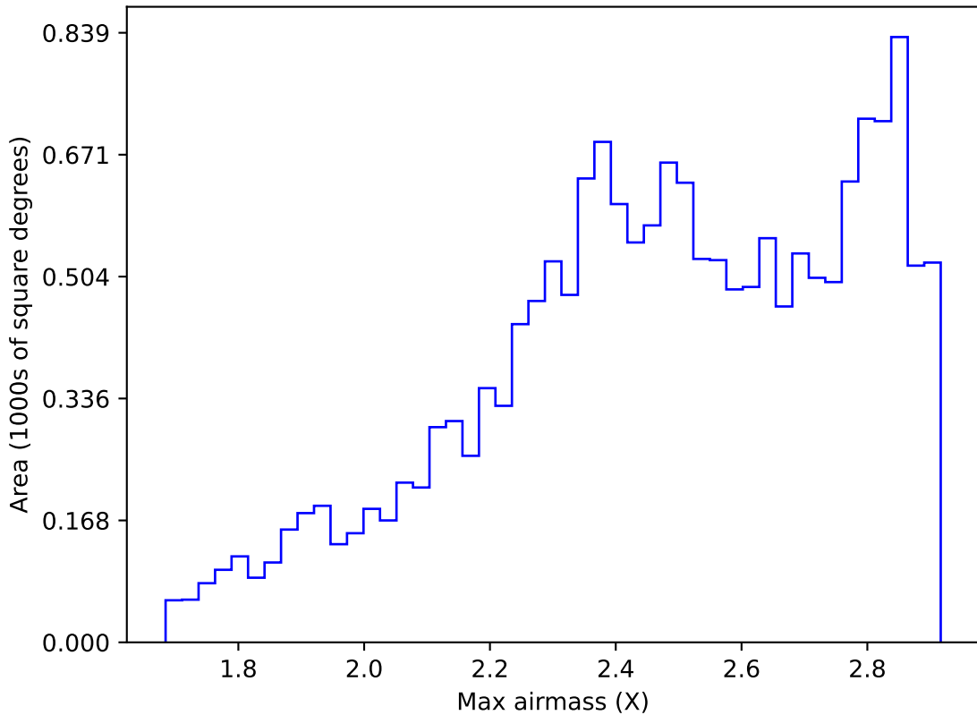
roll_pause_mjdp0_v3.4_10yrs WFD i band: Max airmass
