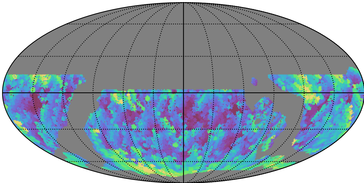
roll_pause_mjdp0_v3.4_10yrs WFD g band: Max airmass
