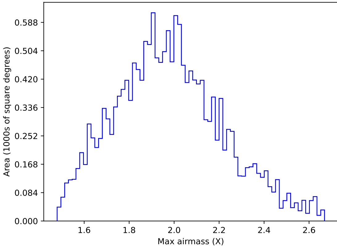
roll_pause_mjdp0_v3.4_10yrs WFD g band: Max airmass
