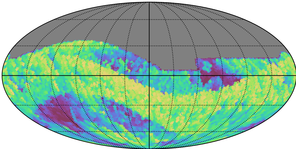
roll_pause_mjdp0_v3.4_10yrs All sky z band: Max airmass
