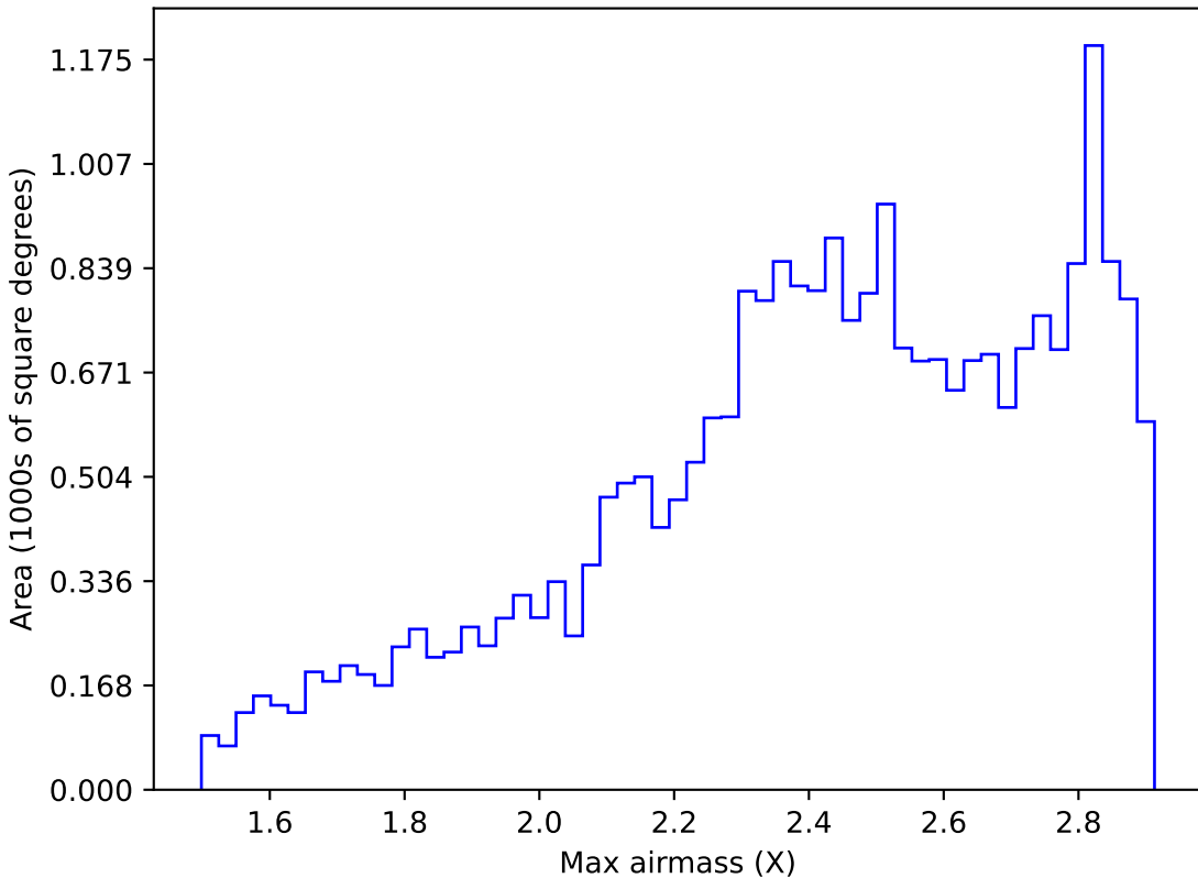
roll_pause_mjdp0_v3.4_10yrs All sky z band: Max airmass
