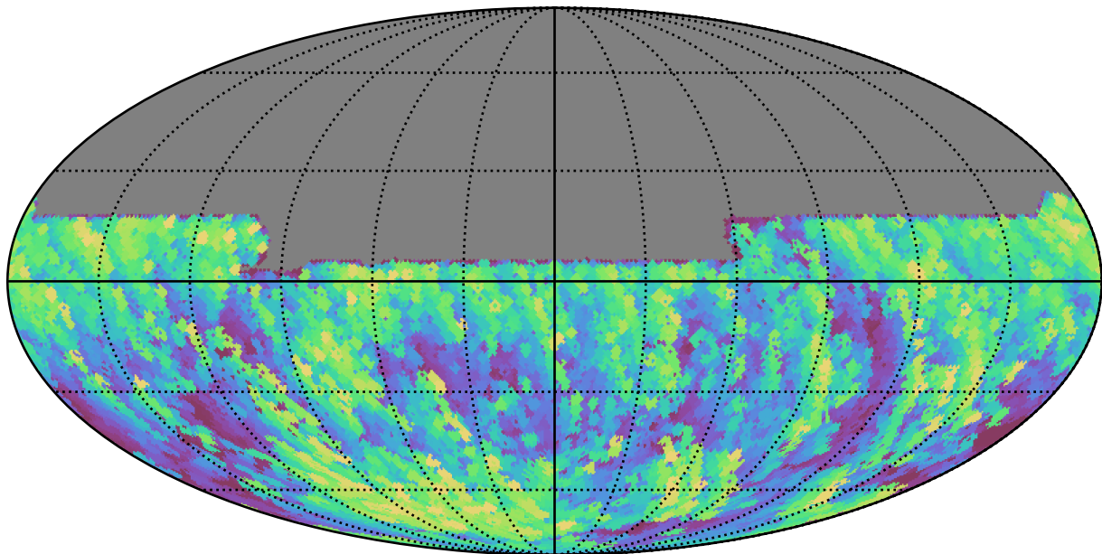
roll_pause_mjdp0_v3.4_10yrs All sky y band: Max airmass
