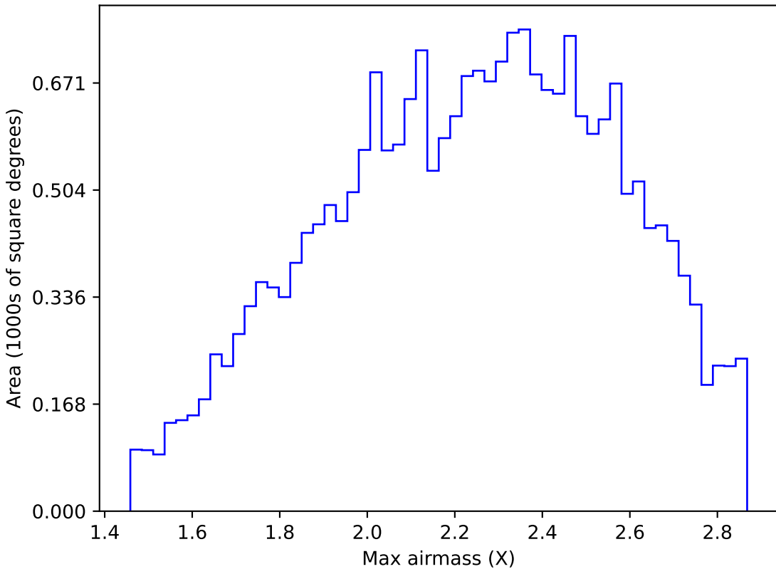
roll_pause_mjdp0_v3.4_10yrs All sky y band: Max airmass
