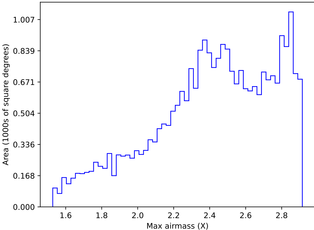
roll_pause_mjdp0_v3.4_10yrs All sky i band: Max airmass
