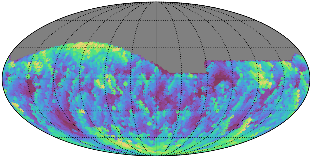
roll_pause_mjdp0_v3.4_10yrs All sky g band: Max airmass
