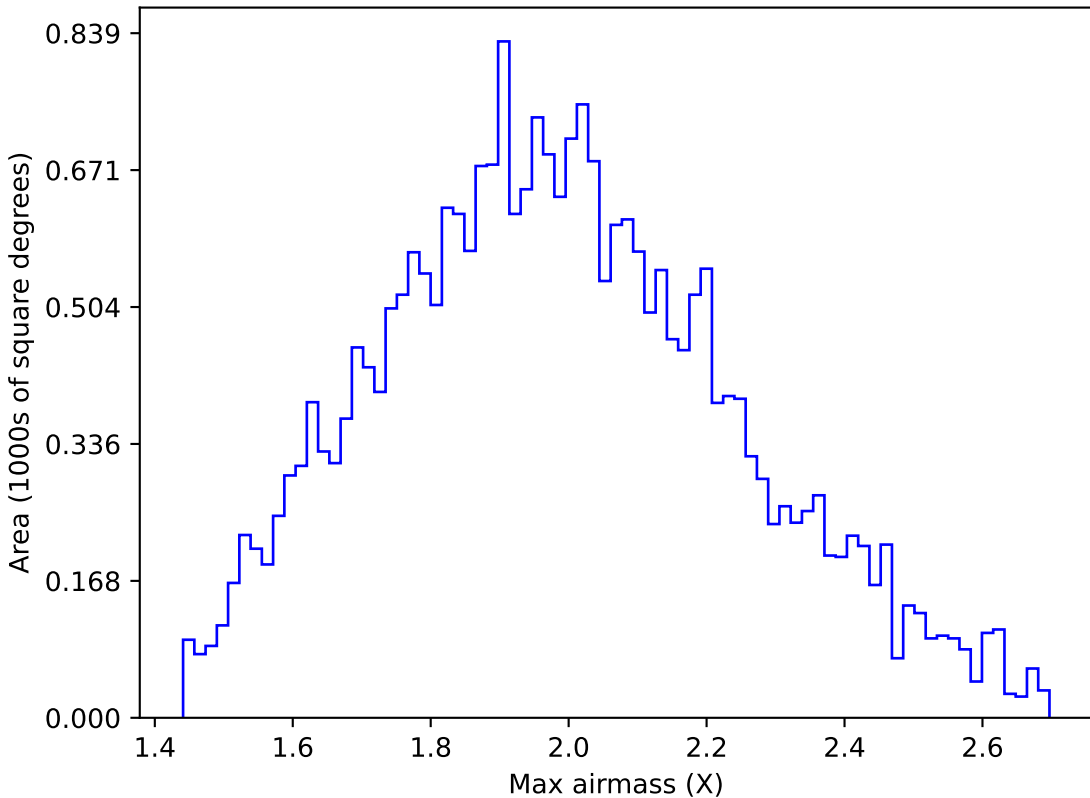
roll_pause_mjdp0_v3.4_10yrs All sky g band: Max airmass
