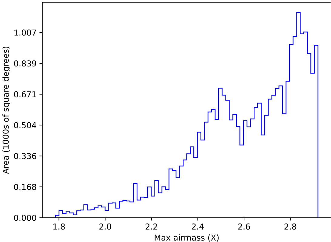
roll_pause_mjdp0_v3.4_10yrs All sky all bands: Max airmass
