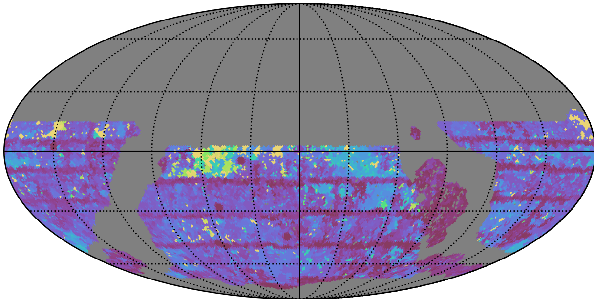
roll_pause_mjdp0_v3.4_10yrs WFD z band: Max Inter-Night Gap
