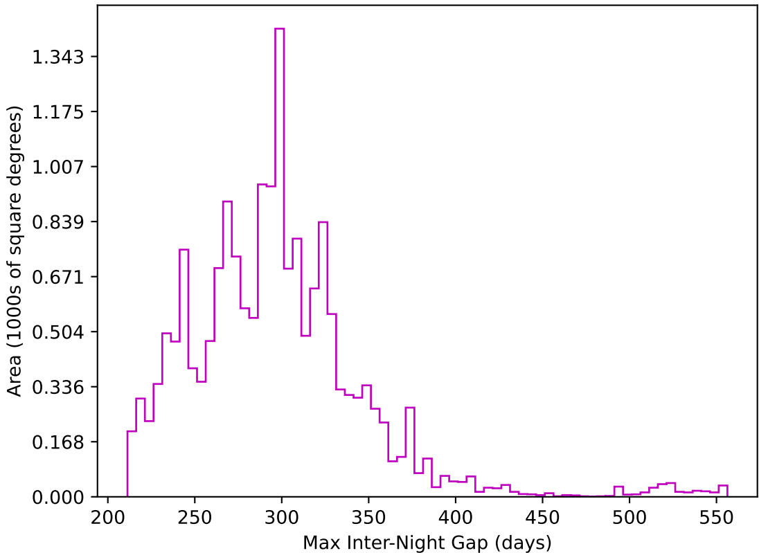
roll_pause_mjdp0_v3.4_10yrs WFD z band: Max Inter-Night Gap
