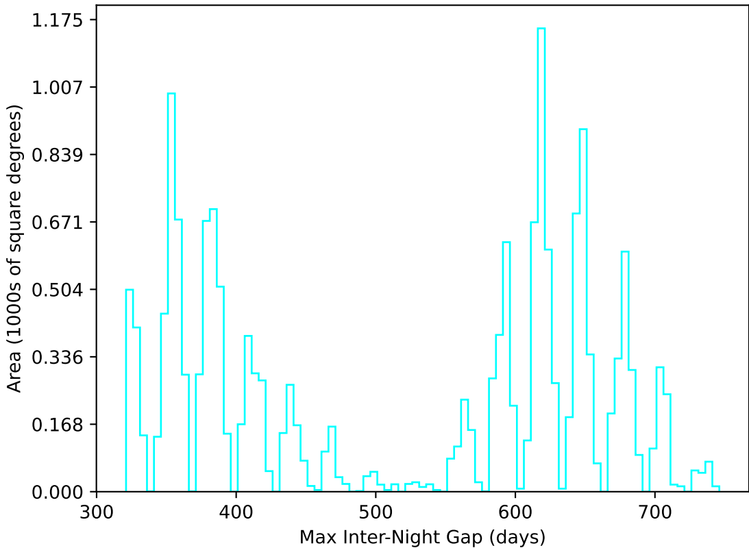
roll_pause_mjdp0_v3.4_10yrs WFD u band: Max Inter-Night Gap
