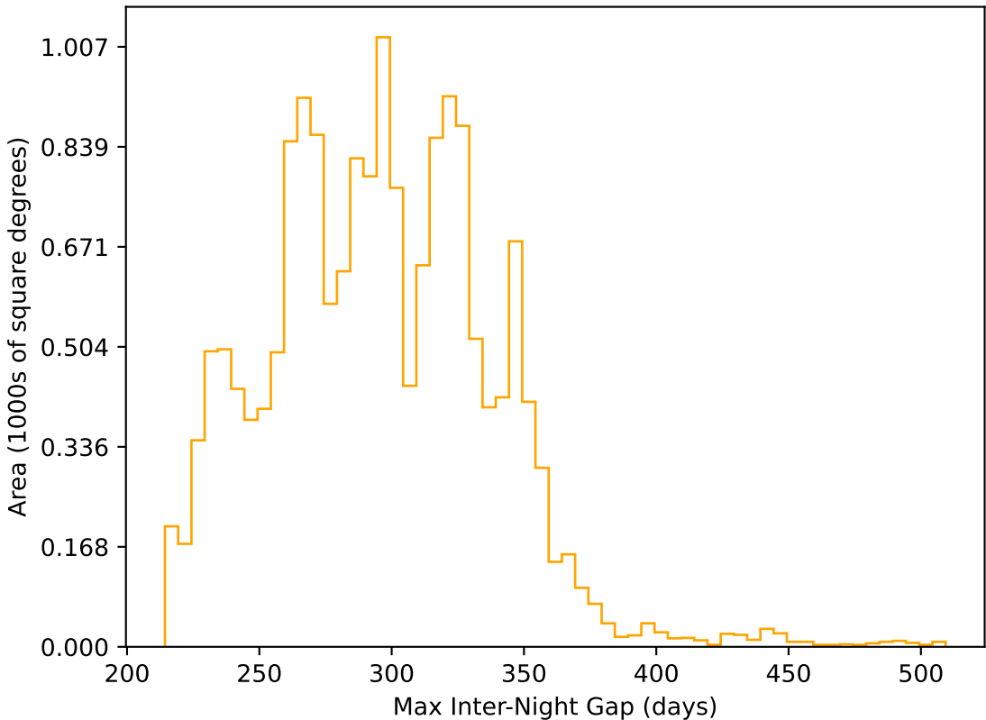
roll_pause_mjdp0_v3.4_10yrs WFD r band: Max Inter-Night Gap
