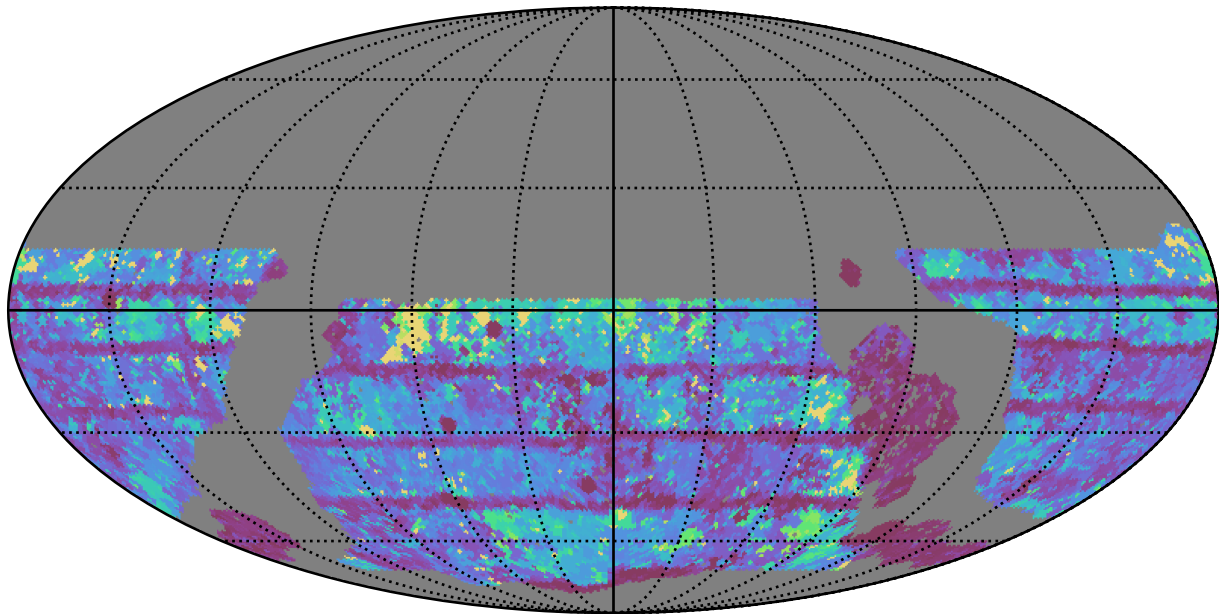
roll_pause_mjdp0_v3.4_10yrs WFD i band: Max Inter-Night Gap
