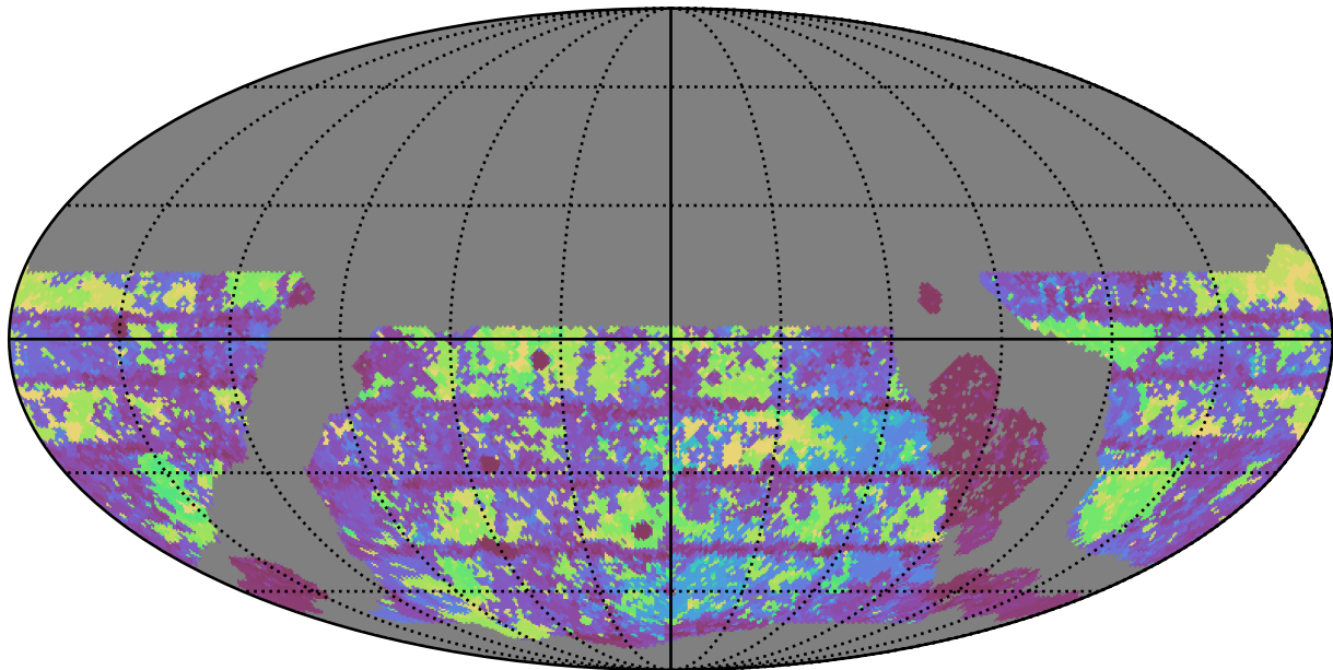
roll_pause_mjdp0_v3.4_10yrs WFD g band: Max Inter-Night Gap
