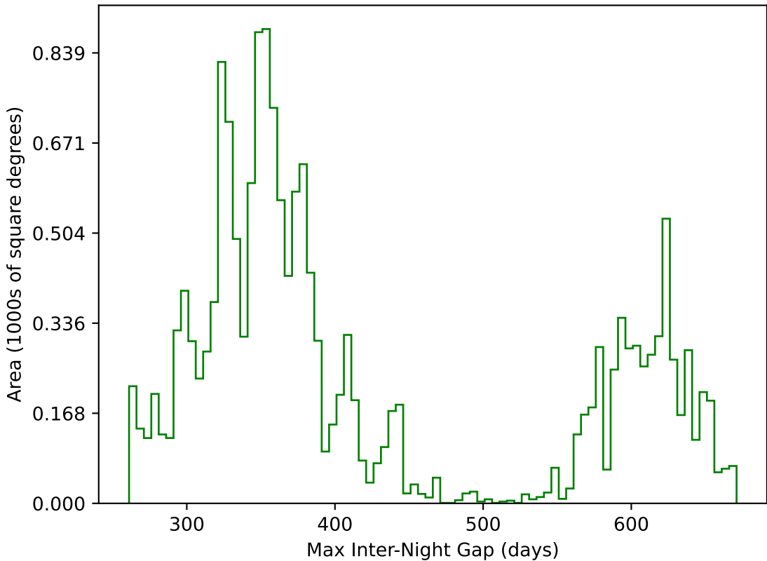
roll_pause_mjdp0_v3.4_10yrs WFD g band: Max Inter-Night Gap
