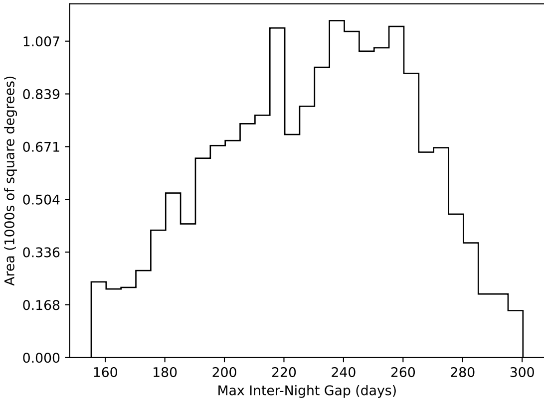
roll_pause_mjdp0_v3.4_10yrs WFD all bands: Max Inter-Night Gap
