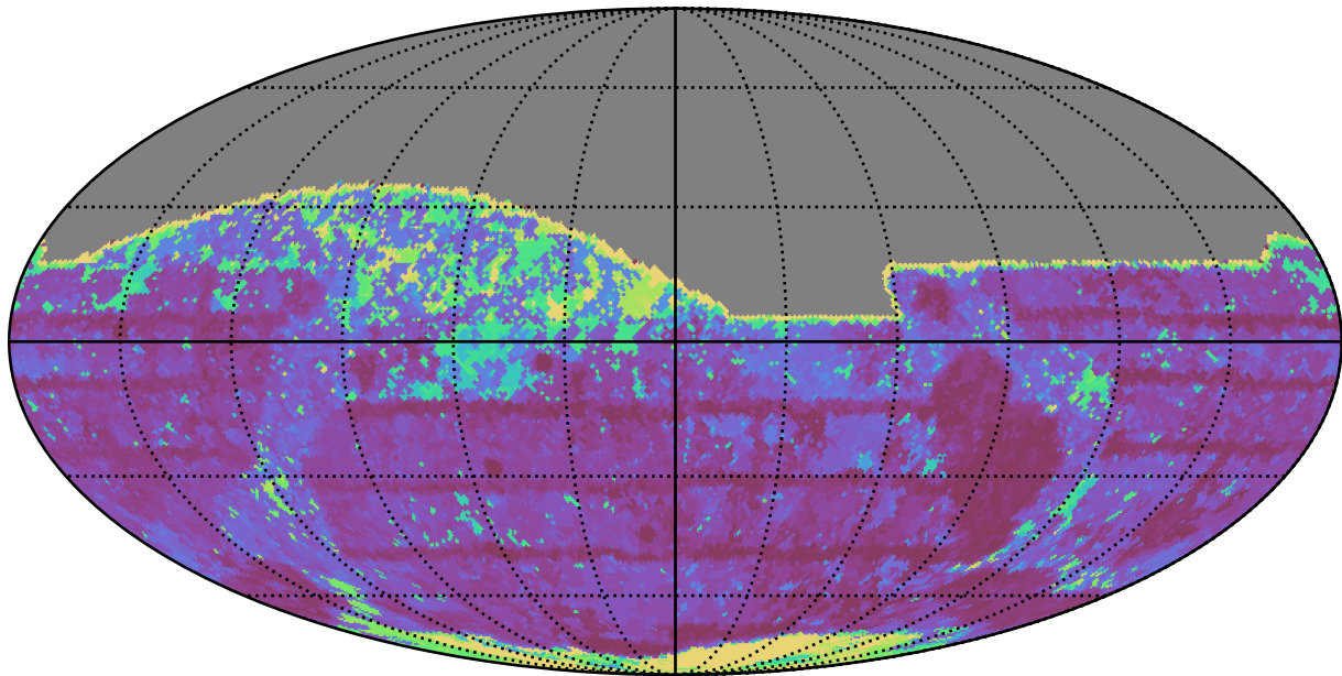
roll_pause_mjdp0_v3.4_10yrs All sky z band: Max Inter-Night Gap
