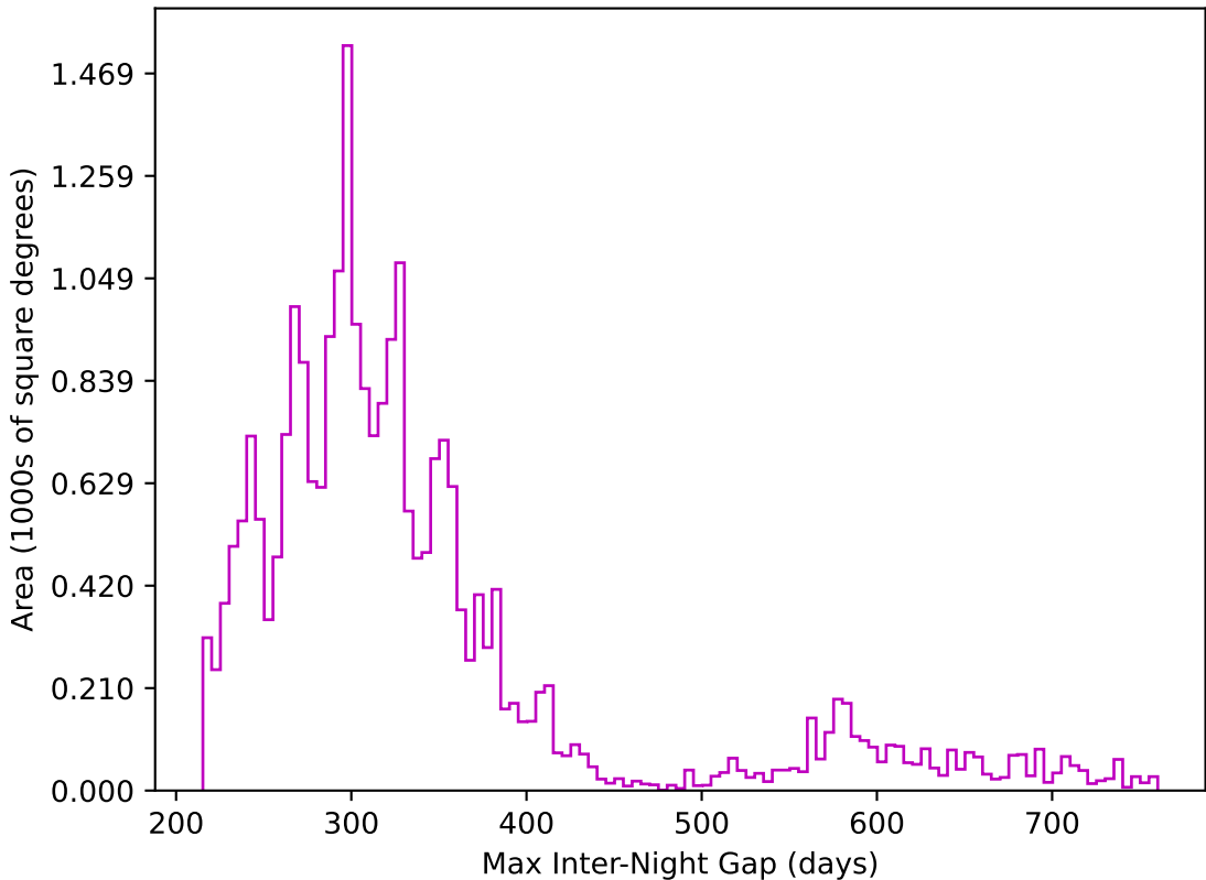
roll_pause_mjdp0_v3.4_10yrs All sky z band: Max Inter-Night Gap
