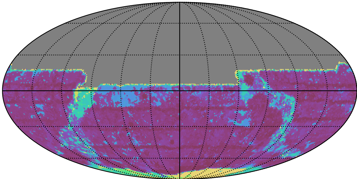
roll_pause_mjdp0_v3.4_10yrs All sky y band: Max Inter-Night Gap
