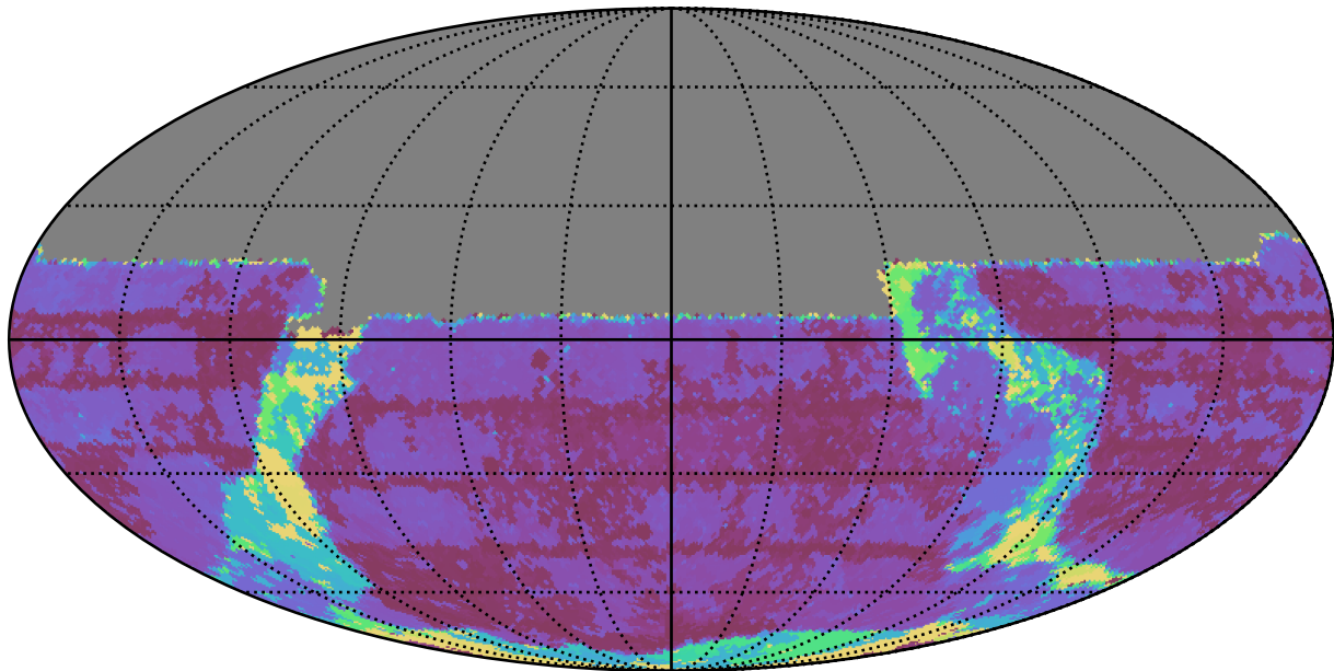
roll_pause_mjdp0_v3.4_10yrs All sky u band: Max Inter-Night Gap
