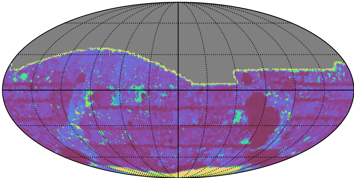
roll_pause_mjdp0_v3.4_10yrs All sky r band: Max Inter-Night Gap
